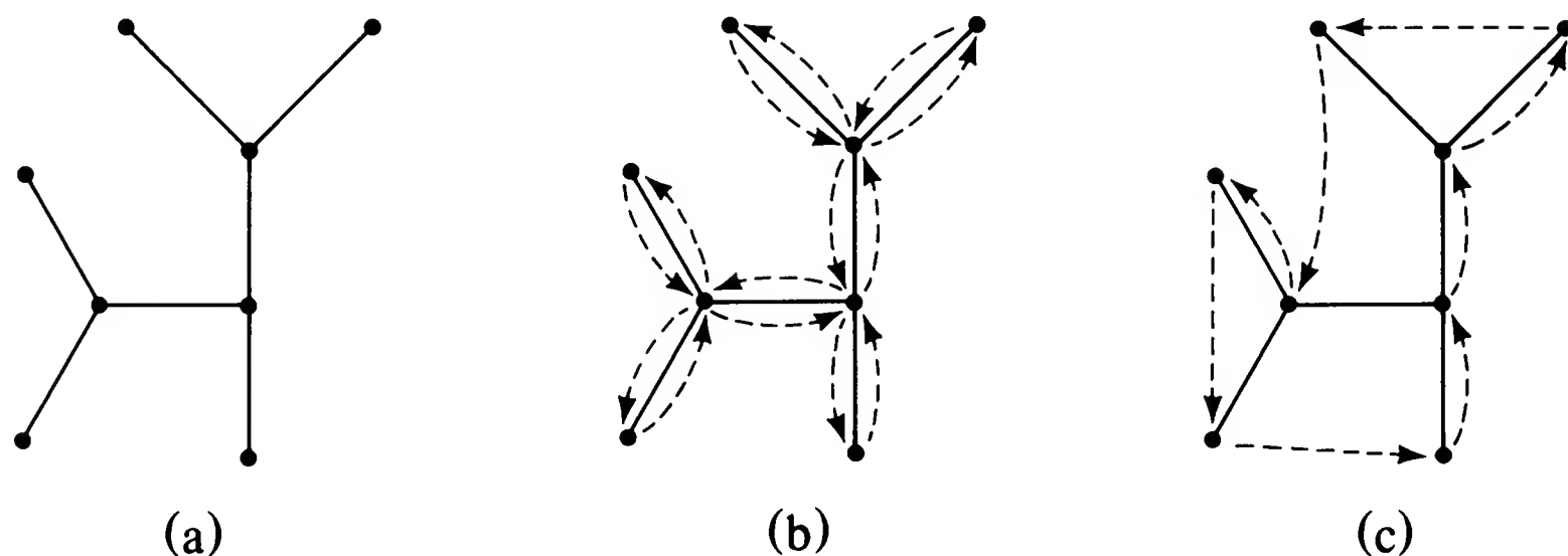
A spanning tree
