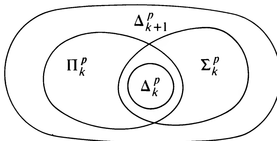
Figure 7.5 Containment relationships within the polynomial hierarchy.
