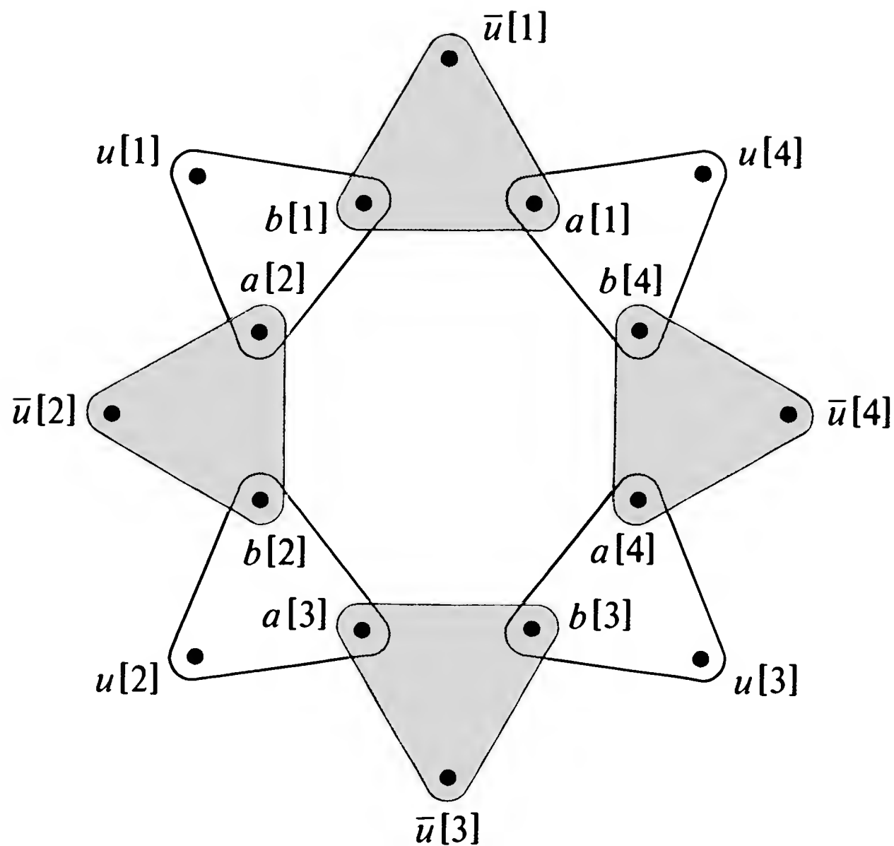
Figure 3.2 Truth setting component T_i when m=4 (subscripts have been deleted for simplicity). Either all the sets of T_i' (the shaded sets) or all the sets of T_i^f (the unshaded sets) must be chosen, leaving uncovered all the u_i[j] or all the \bar{u}_i[j] , respectively.
