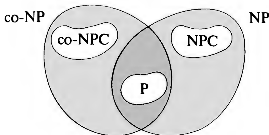
Figure 7.2 The world of NP and vicinity (assuming P \neq NP and NP \neq co-NP ). It may or may not be the case that P = NP \cap co-NP .
