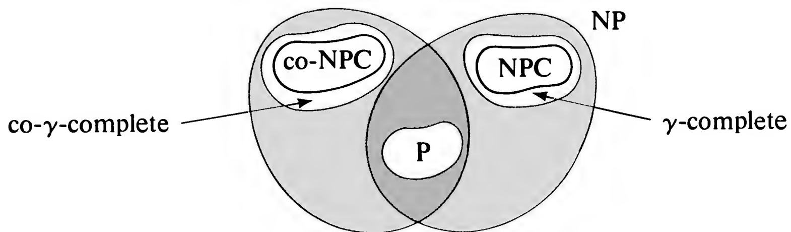
Figure 7.3 The world of NP, once more revised (assuming that both P \neq NP and NP \neq \text{co-NP} ).
