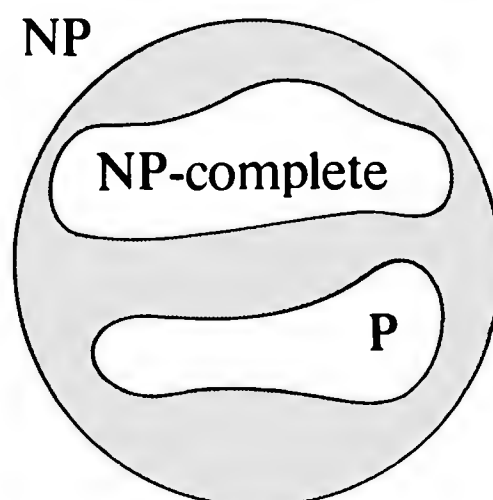
Figure 2.6 The world of NP, revisited.
